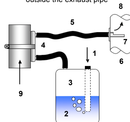
Reactor Retrokit ® Nano-Pro, installed outside the exhaust pipe
